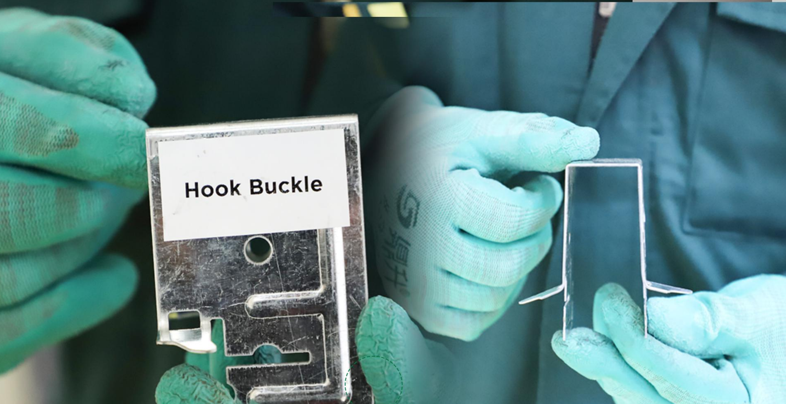
9、 Assemble hook buckle - bend the side pieces as shown
